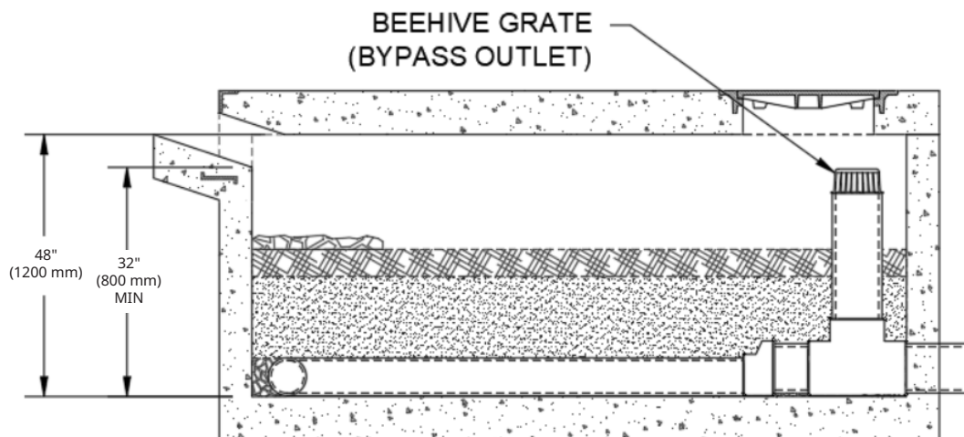
Figure 4: EcoStream inlet/outlet
