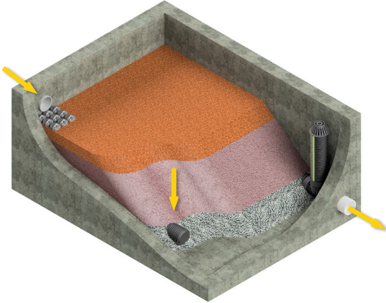
Figure 2: Treatment flow path shown through a unit with an inlet pipe
