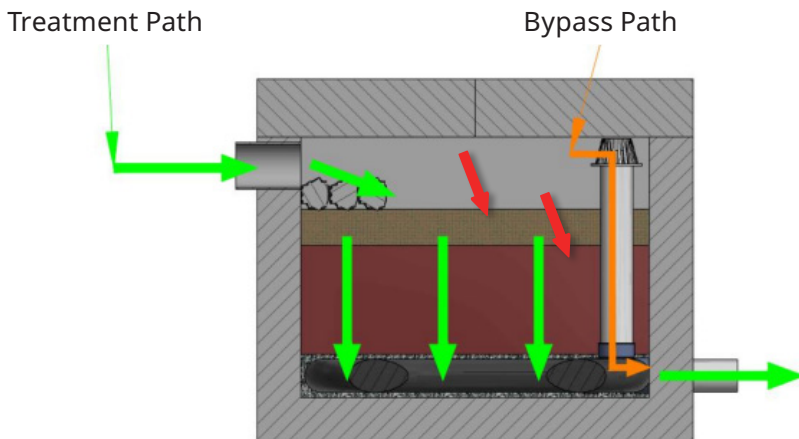
Figure 3: Treatment flow pathway shown in profile view
