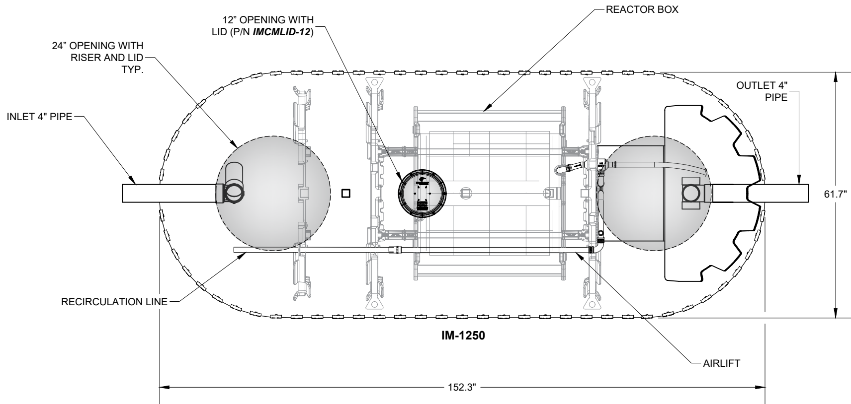
PLAN VIEW
