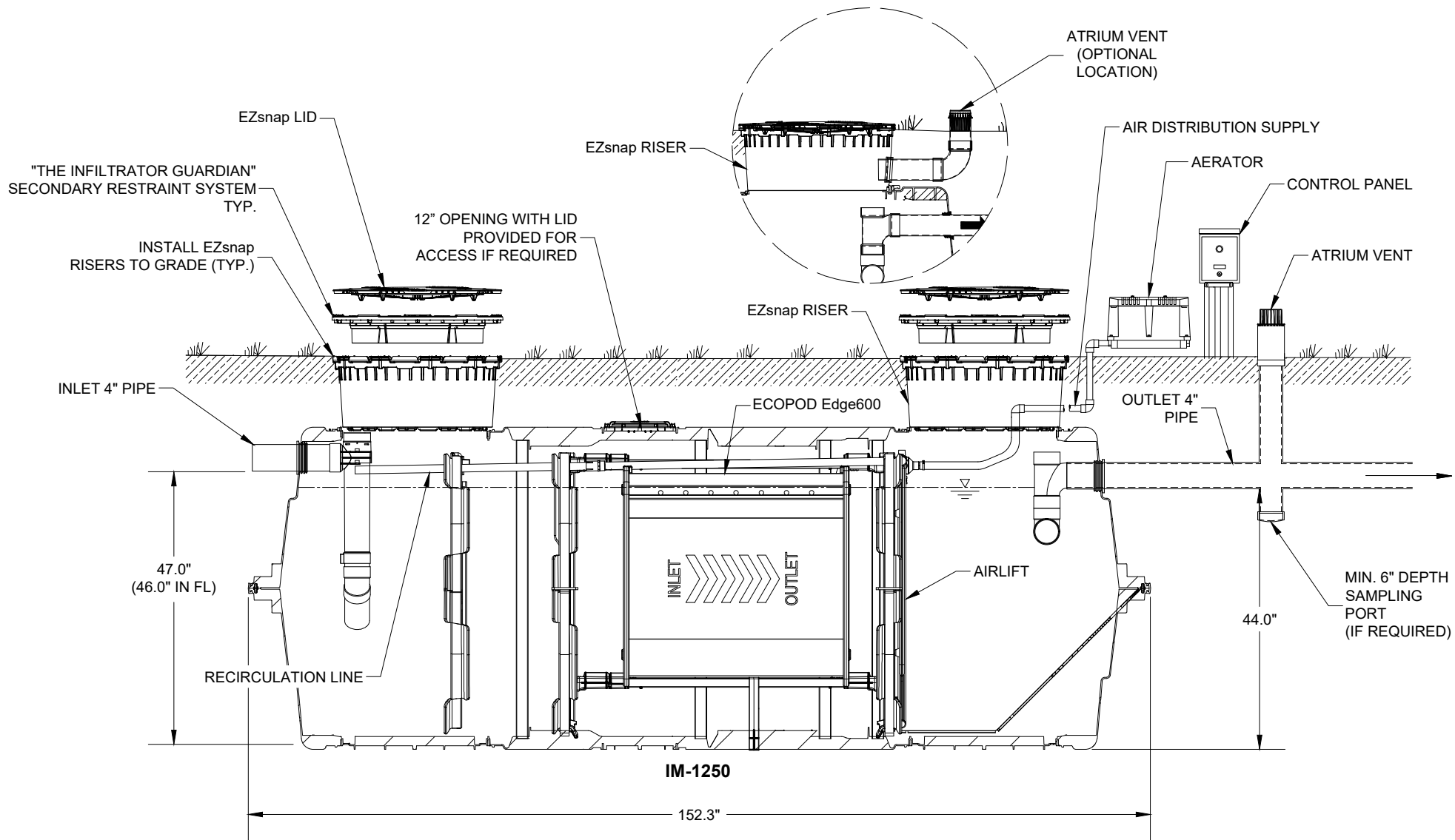
CROSS SECTION
