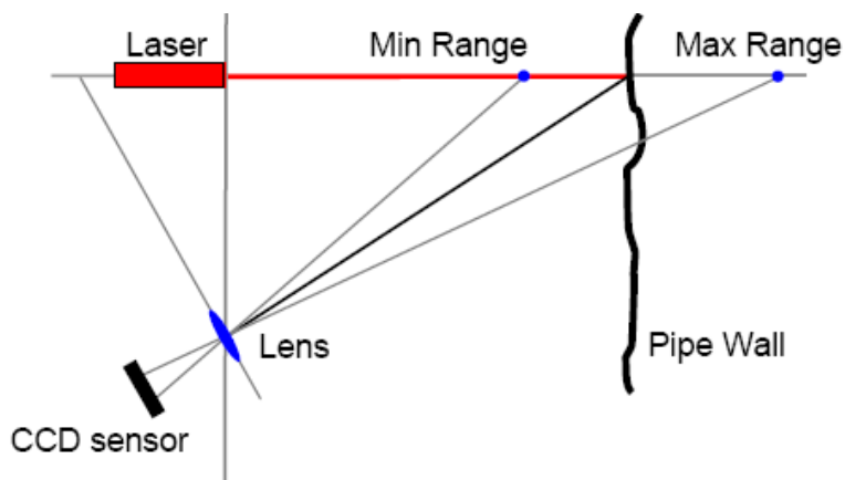
Figure 1: Optical Triangulation Geometry
