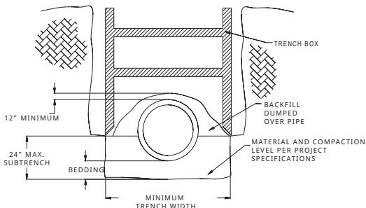
Figure 2: Subtrench Installation
