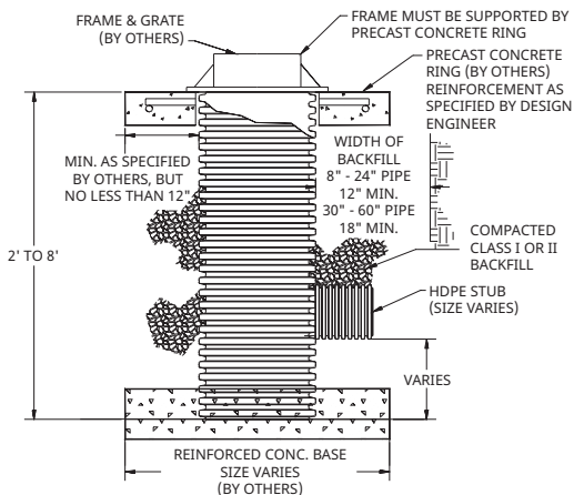
Figure 6: Vertical Riser
