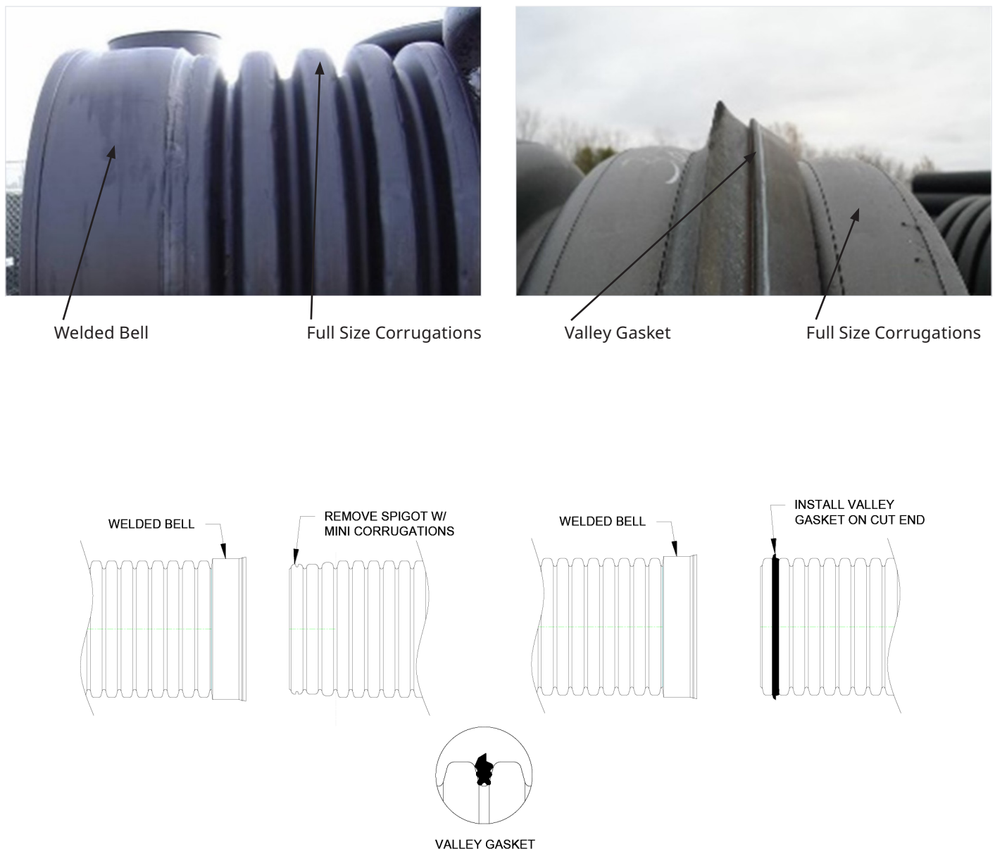
Figure 2: Welded Bell Connection
