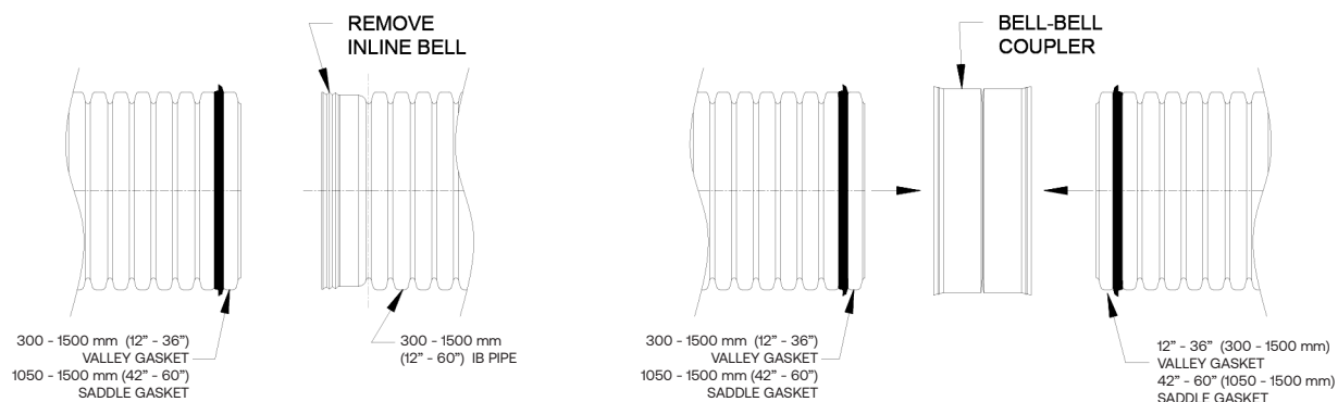
Figure 3: Bell-Bell Coupler Connection
