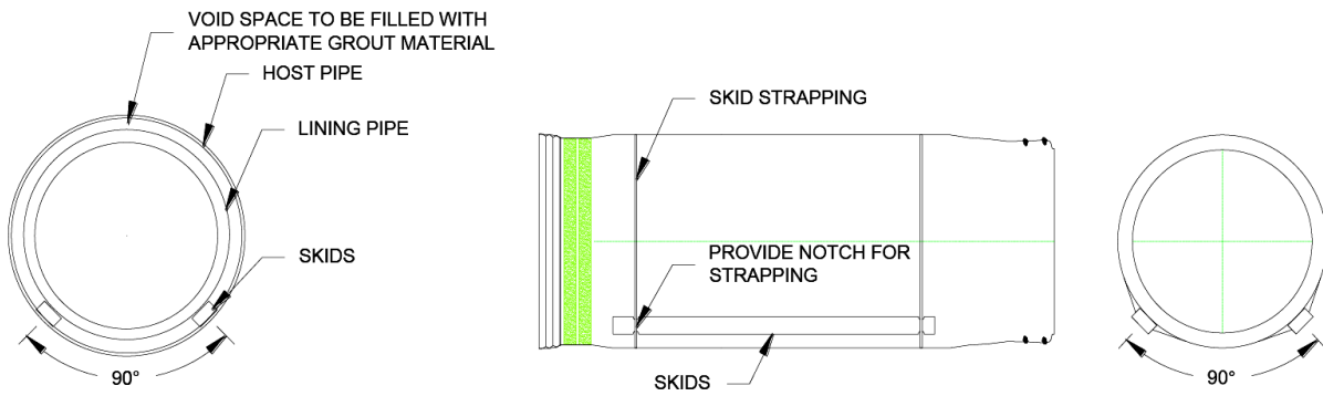
Figure 1: Attachment of Skids to HP Pipe
