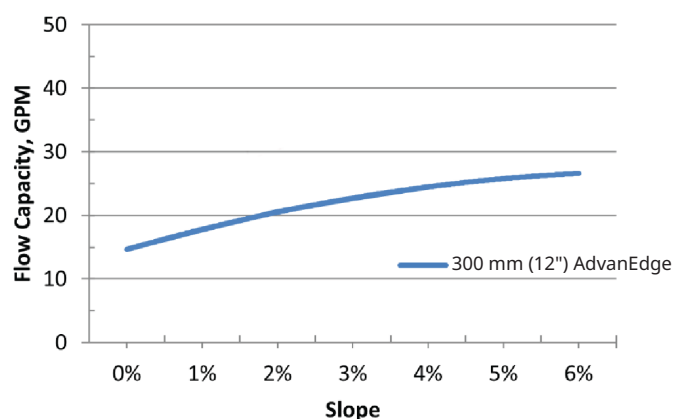
Figure 1: AdvanEdge Core Flow Capacity Horizontal Plane Installation
