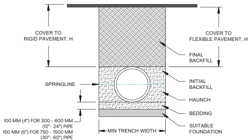
Figure 1: HP Storm Pipe Trench Detail with Uniform Backfill (Traffic and Non-Traffic Applications)
