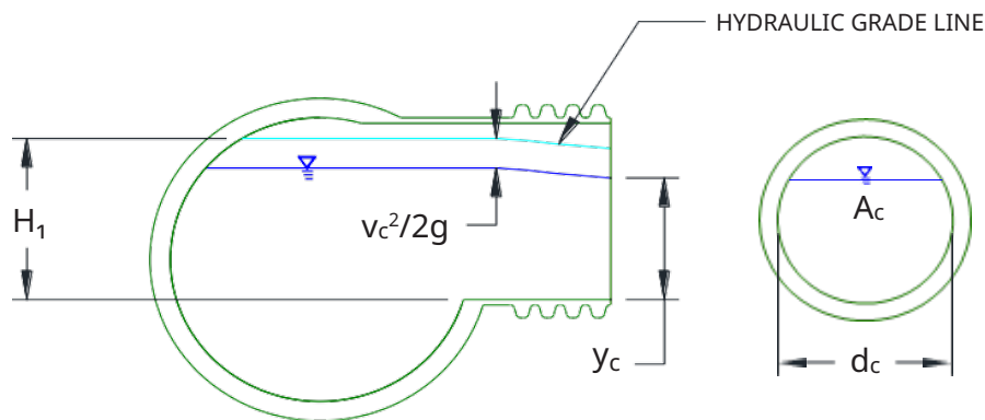
Figure 2: StormTech Manifold as a Broad-Crested Weir with Circular Cross Section
