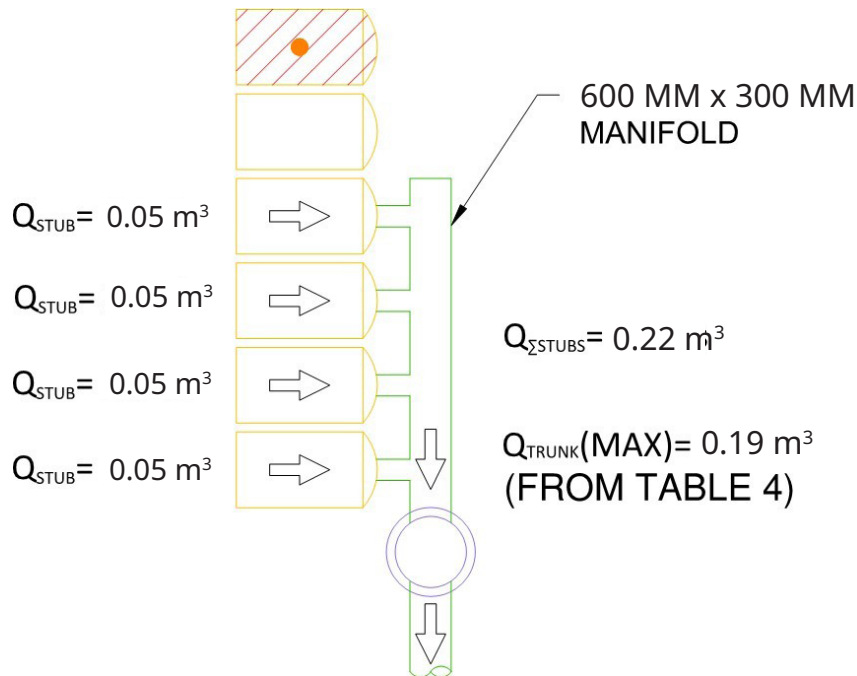
Figure 4: Determining Maximum Allowable Outlet Flow for Reducing Manifolds
