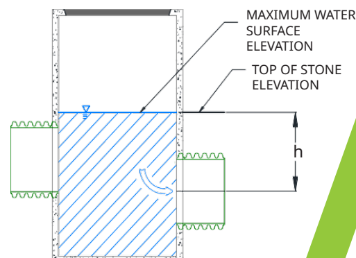
Figure 1: Head for Orifice of a Short Tube Equation
