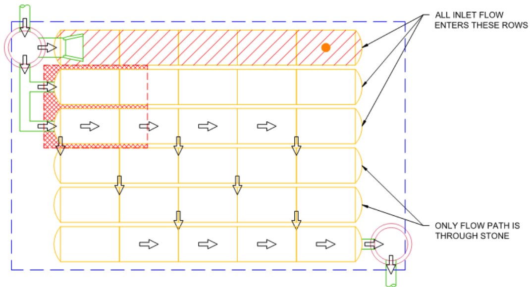
Figure 5: Flow Path through StormTech Systems based on Manifold Configuration
