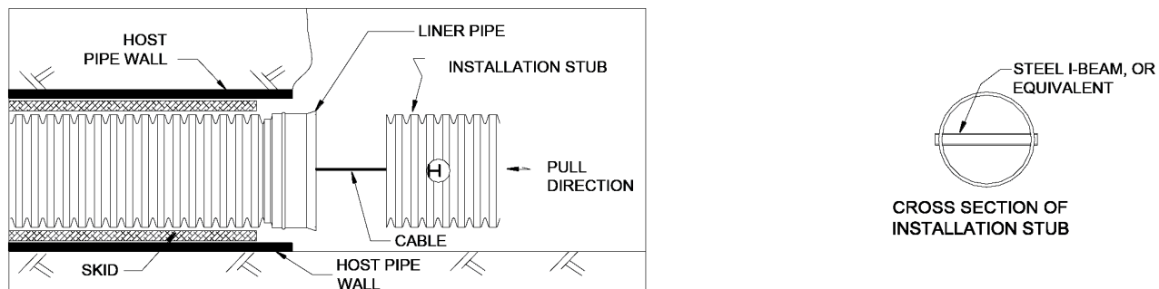
Figure 3: Installation of Liner Pipe using Installation Stub
