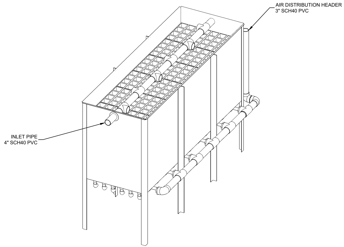
ECOPOD REACTOR LAYOUT 1
