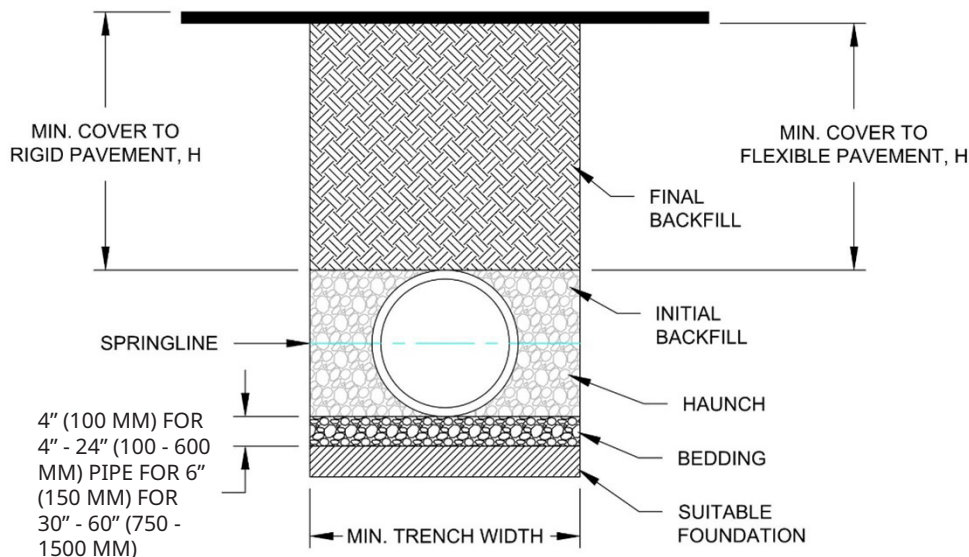
Figure 1 SaniTite HP Trench Detail (Sanitary Sewer)
