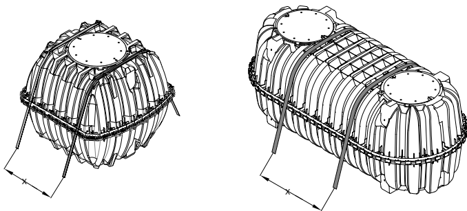
Figure 10: Strap Positioning
