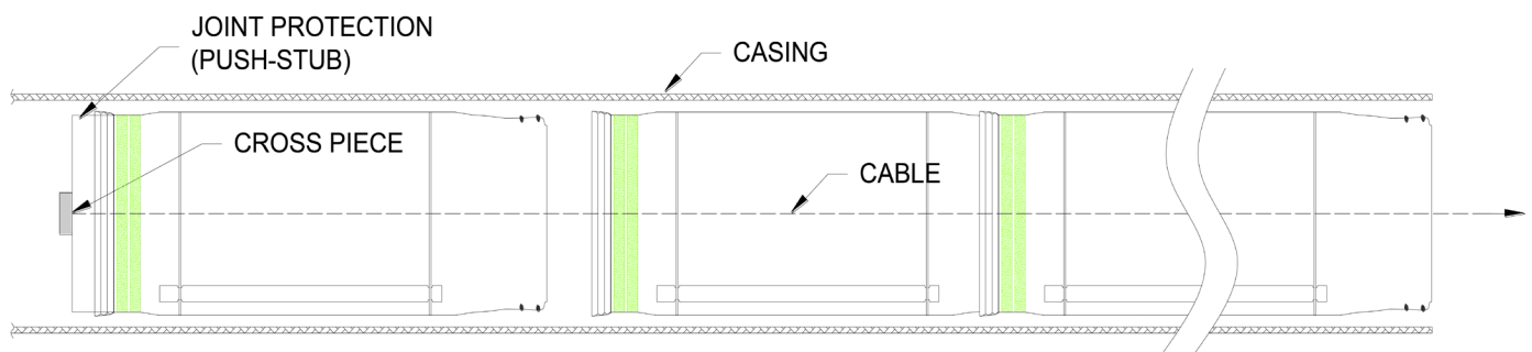
Figure 3: Alternative Installation Method (Used when maximum insertion forces are likely to be exceeded)
