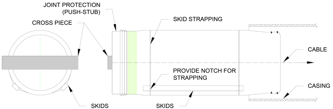
Figure 2 : Pulling SaniTite HP Pipe in Casing
