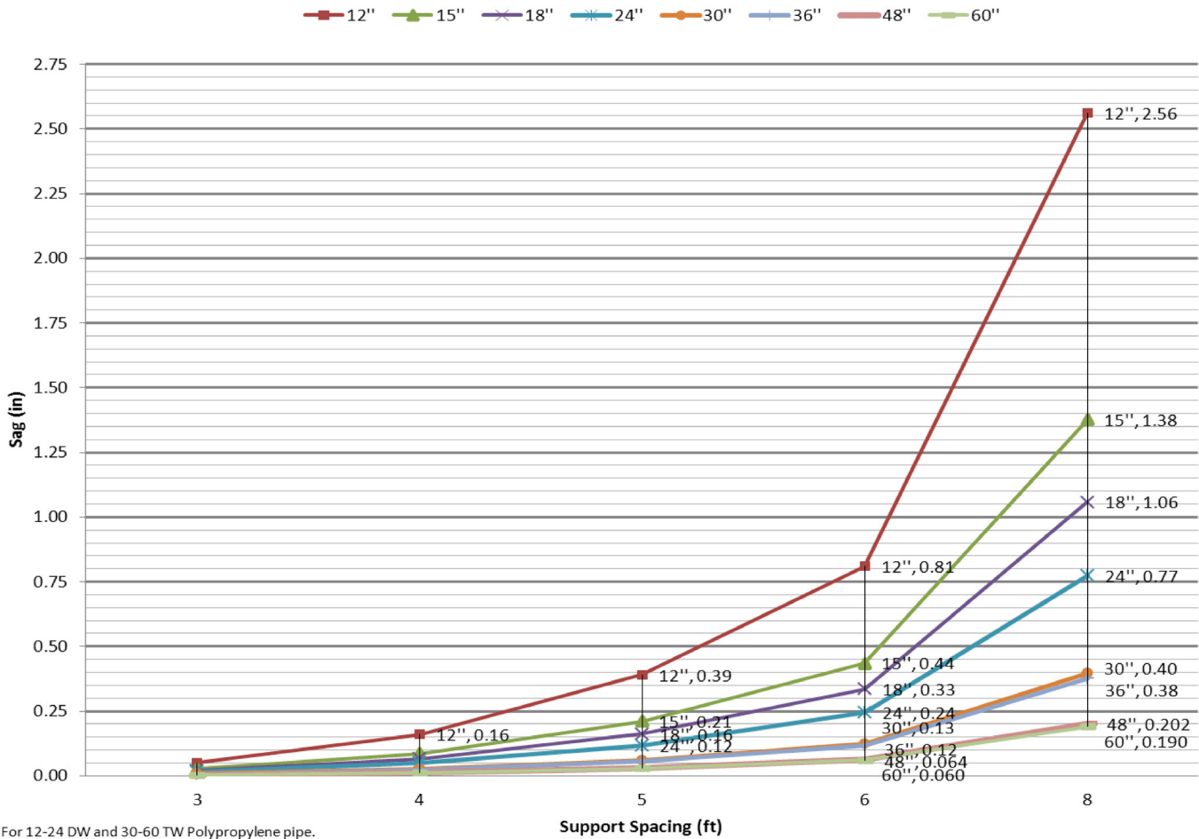
Chart 1 : Unsupported Deflection of SaniTite HP
