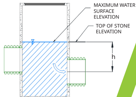
Figure 1: Head for Orifice of a Short Tube Equation
