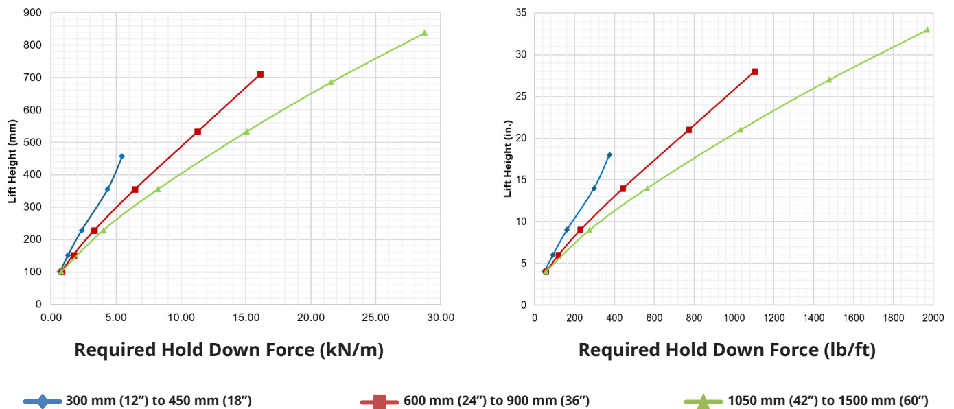
Figure 1: Hold Down Force for Incremental Lifts
