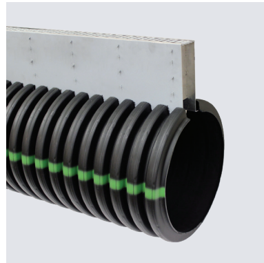
Duraslot Slotted Drains
