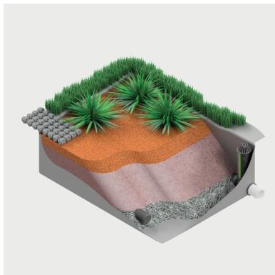
EcoStream™ BioFilter (Lined System)
