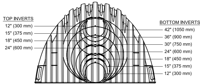
Figure 8—MC-4500 End Cap Inverts
