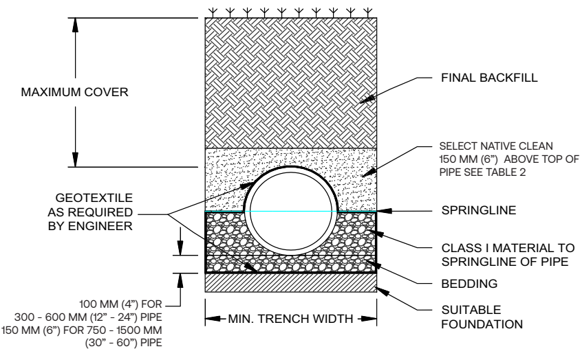
Figure 1: HP Storm Pipe Trench Detail with Uniform Backfill (Traffic and Non-Traffic Applications)
