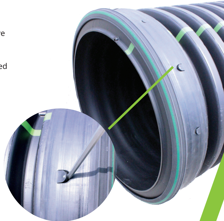
Pictured above is a 600-900 mm (24"-36") saddle gasket.
