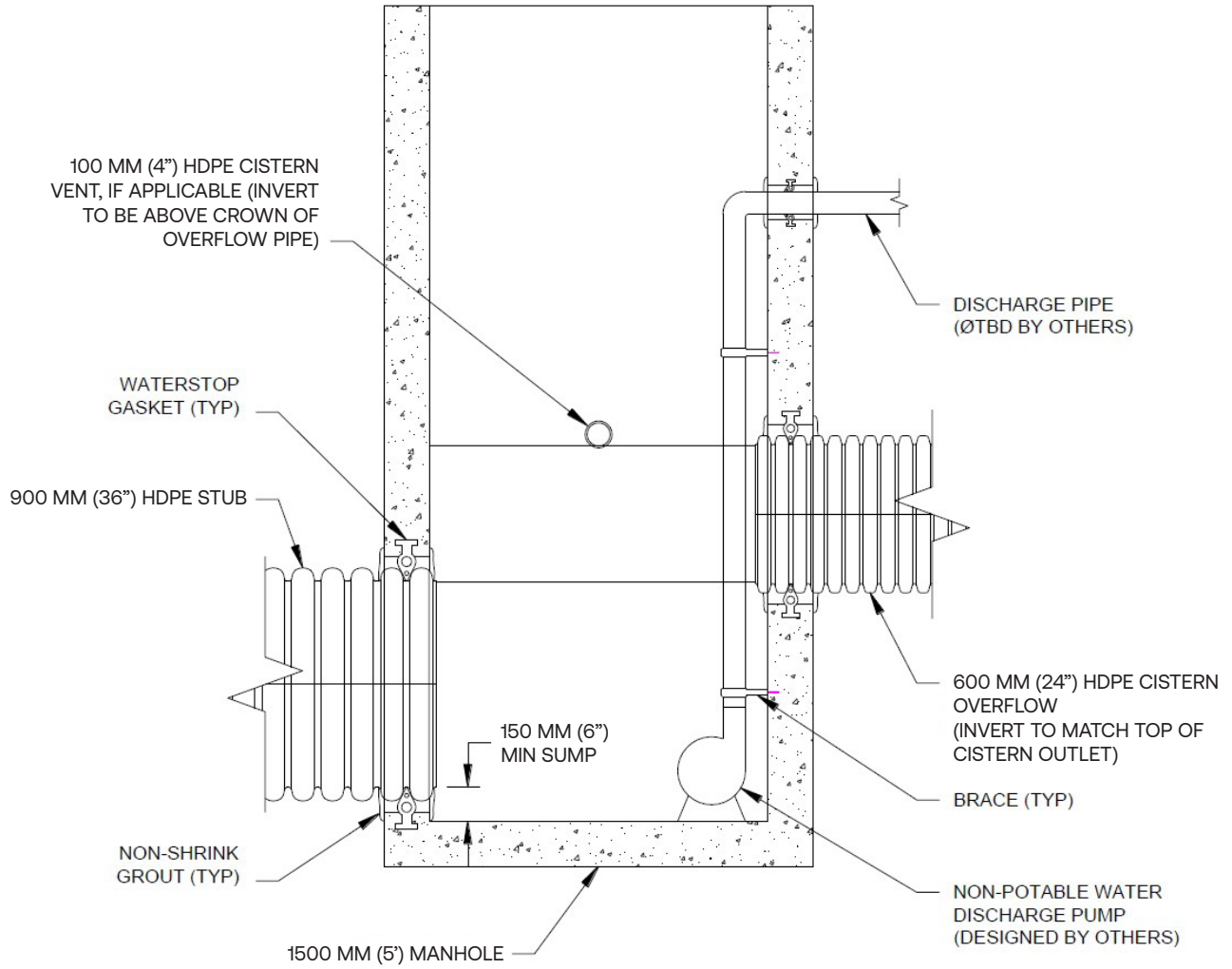
Figure 2: Outlet Manhole Typical Detail
