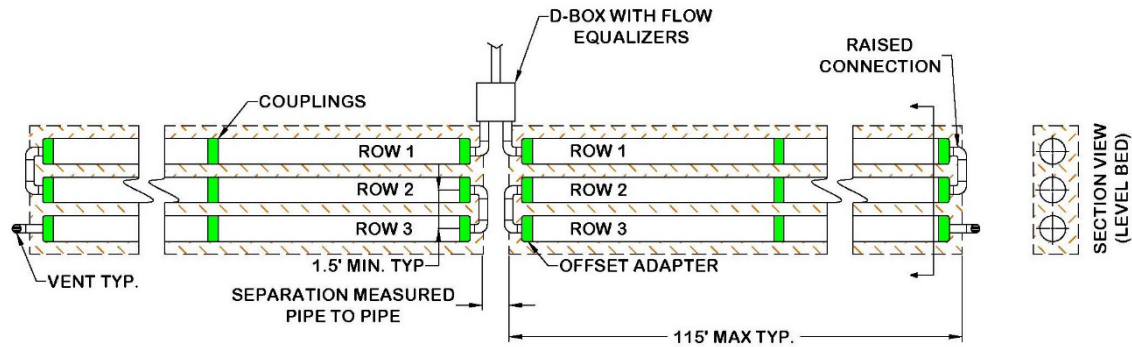
Illustration of Side-to-Side Multiple Beds:
