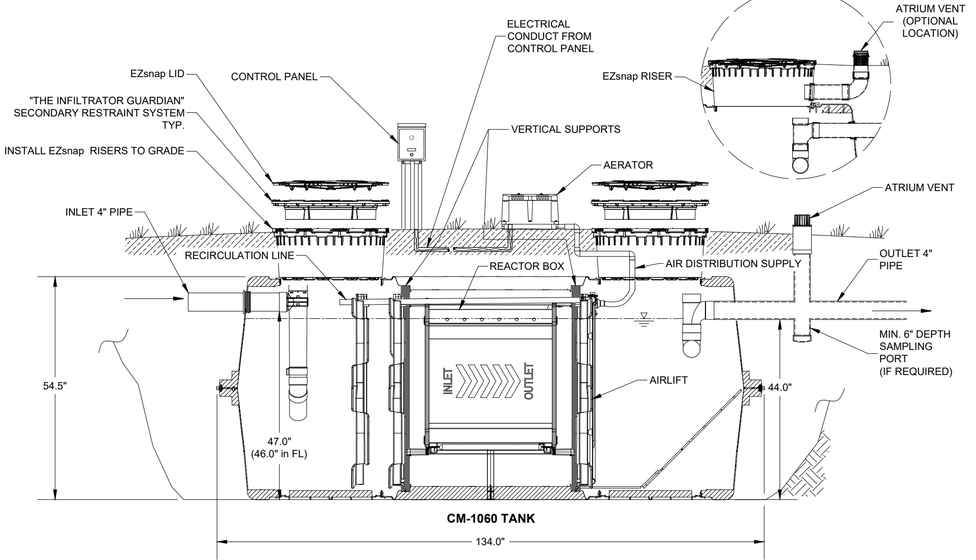
CROSS SECTION
