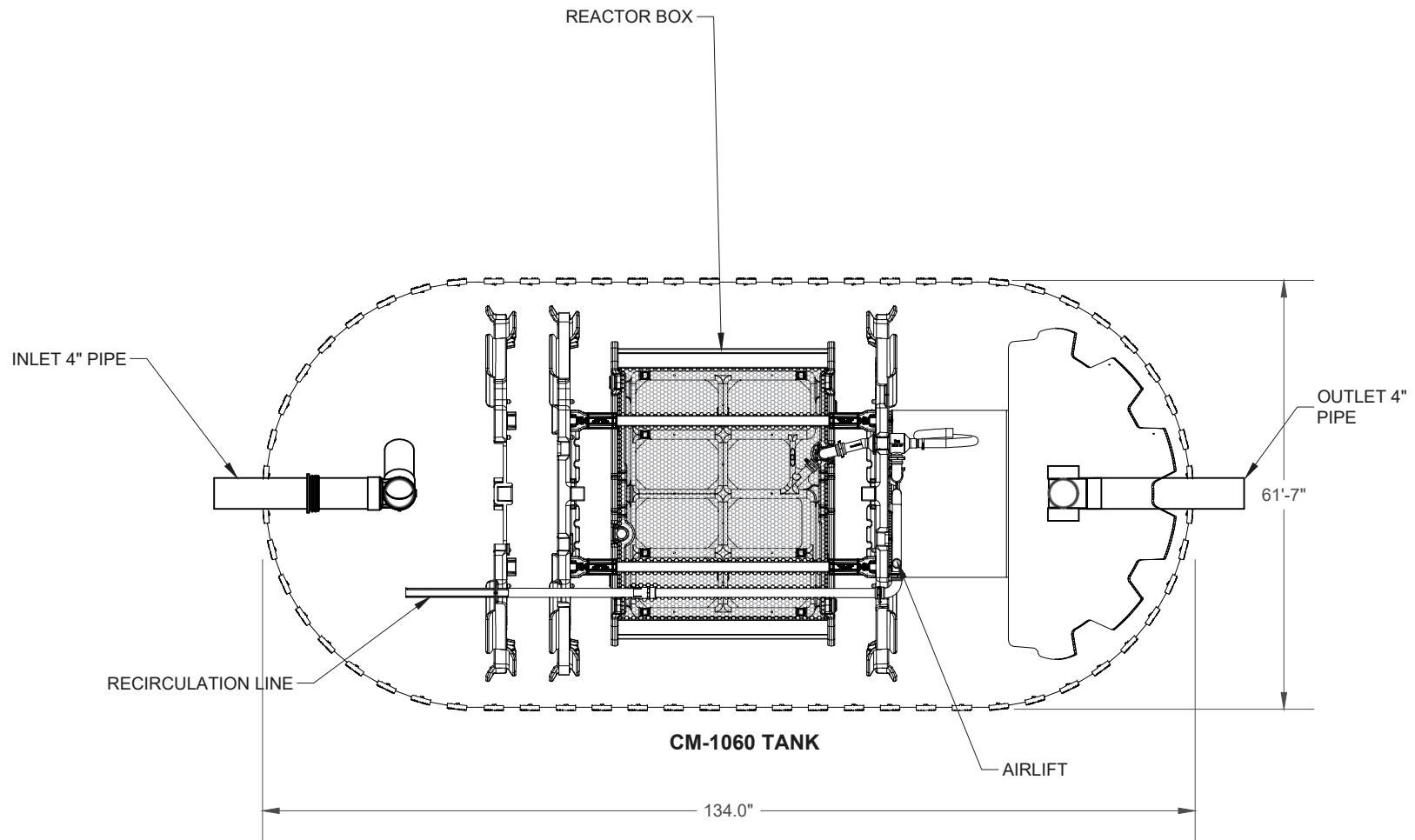
PLAN VIEW
