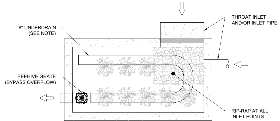
ECOSTREAM OPEN TOP PLAN VIEW
