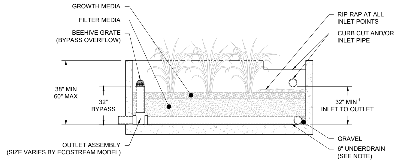
ECOSTREAM OPEN TOP PROFILE VIEW
