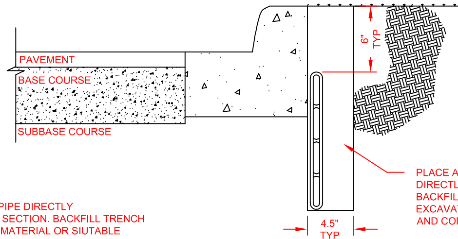
ADVANEDGE INSTALLATION DETAIL (CITY STREET W/ CURB & GUTTER)
