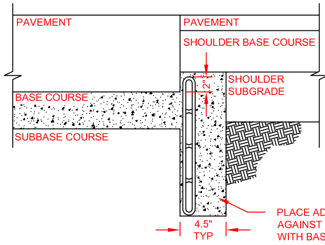
ADVANEDGE INSTALLATION DETAIL (NO CURB & GUTTER)
