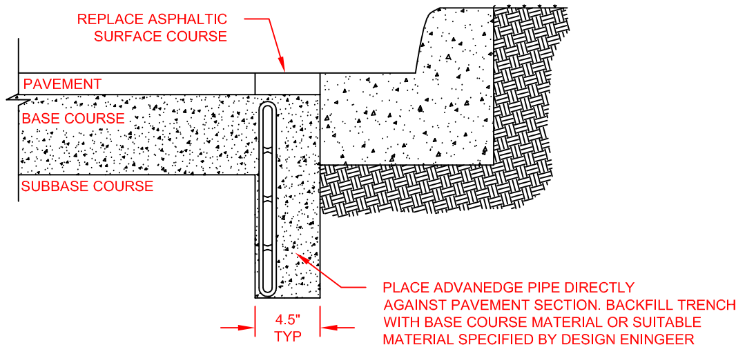
ADVANEDGE INSTALLATION DETAIL (CITY STREET W/ CURB & GUTTER)
