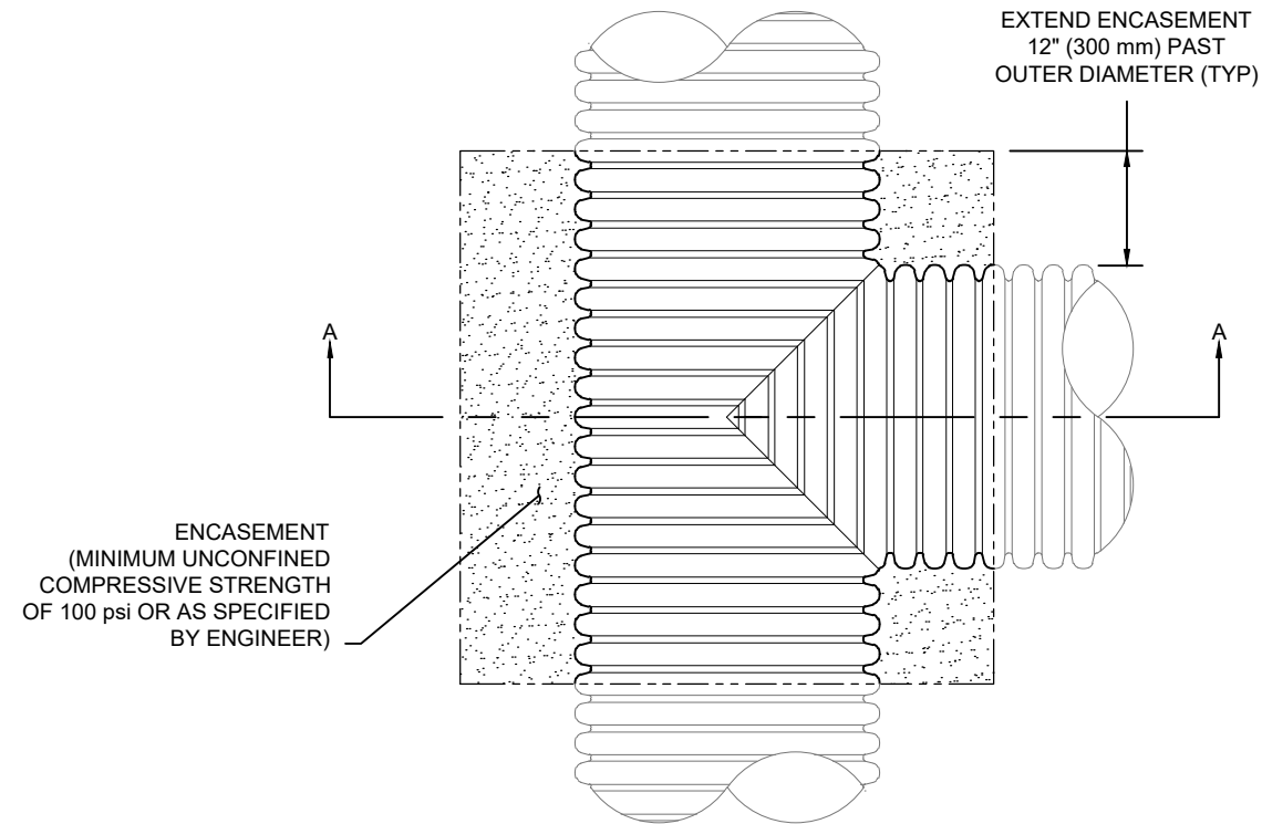
PLAN VIEW
