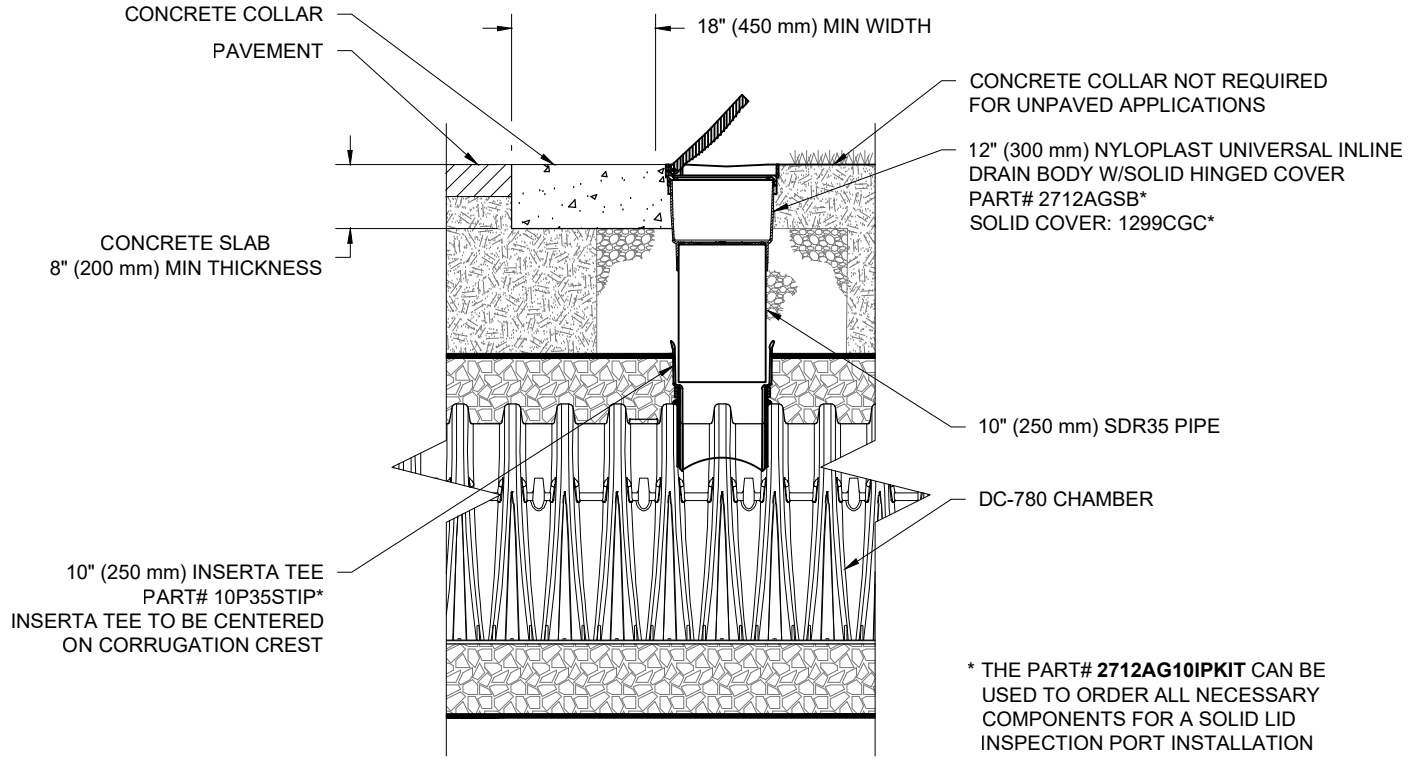
DC-780 10" (250 mm) INSPECTION PORT DETAIL
