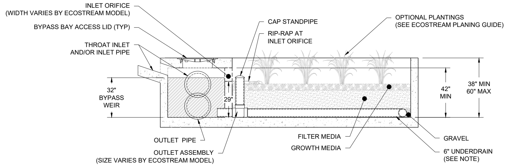
ECOSTREAM OPEN TOP PROFILE VIEW NOT TO SCALE
