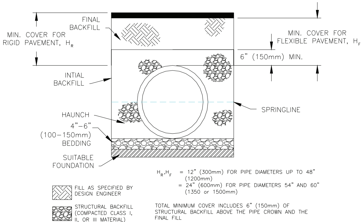
Figure 1 Typical Backfill Structure
