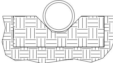
2 (b) Trapezoidal Bottom 8" - 24" (200 mm - 600 mm)
