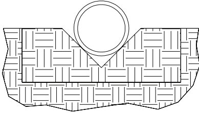
2 (a) "V" Groove 4" - 8" (100 mm - 200 mm)
