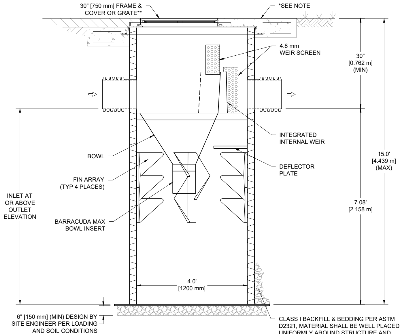
SECTION VIEW A-A NOT TO SCALE
