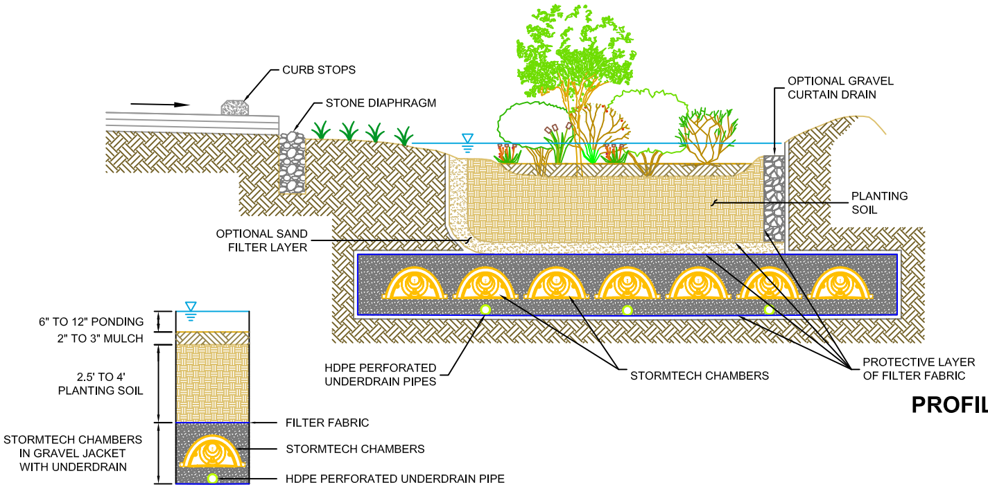
TYPICAL SECTION
