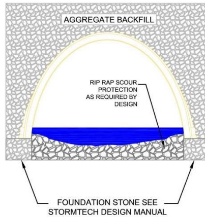
AGGREGATE FOOTING OPTION 2: AGGREGATE BOTTOM (FOR LOW FLOW APPLICATIONS)
