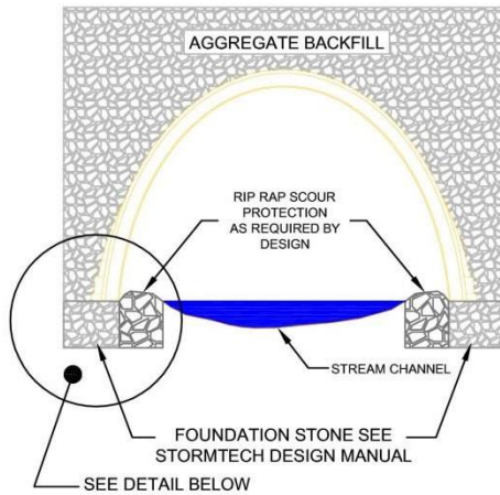
AGGREGATE FOOTING OPTION 1: OPEN BOTTOM (FOR VERY LOW FLOW APPLICATIONS)
