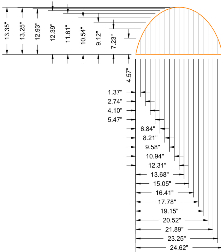
Figure 7 SC-310 User Defined Shape
