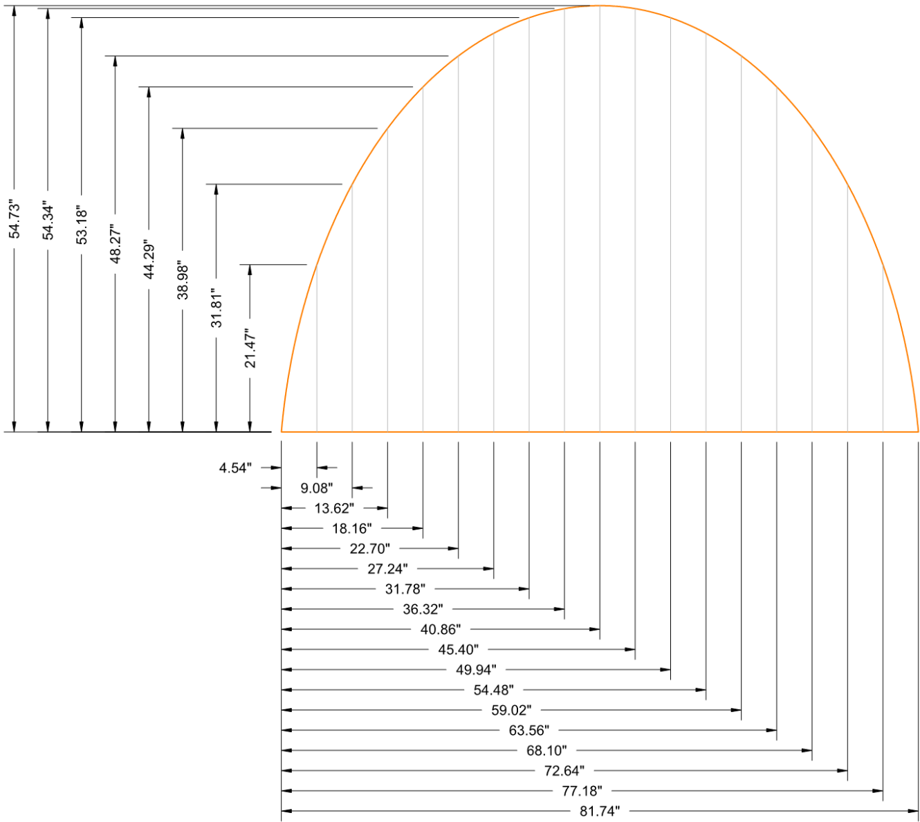
Figure 4 MC-7200 User Defined Shape
