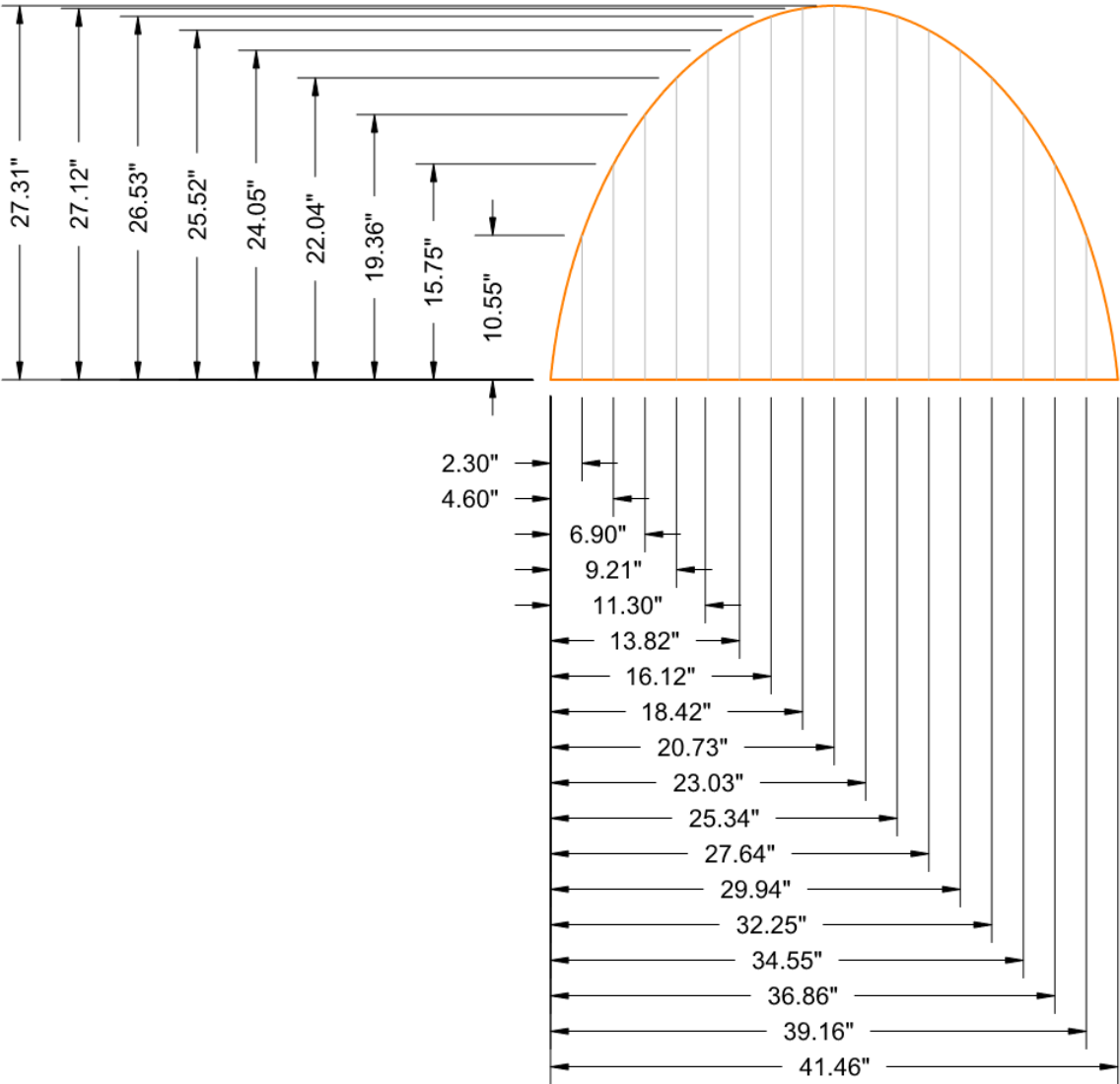
Figure 6 SC-740 User Defined Shape
