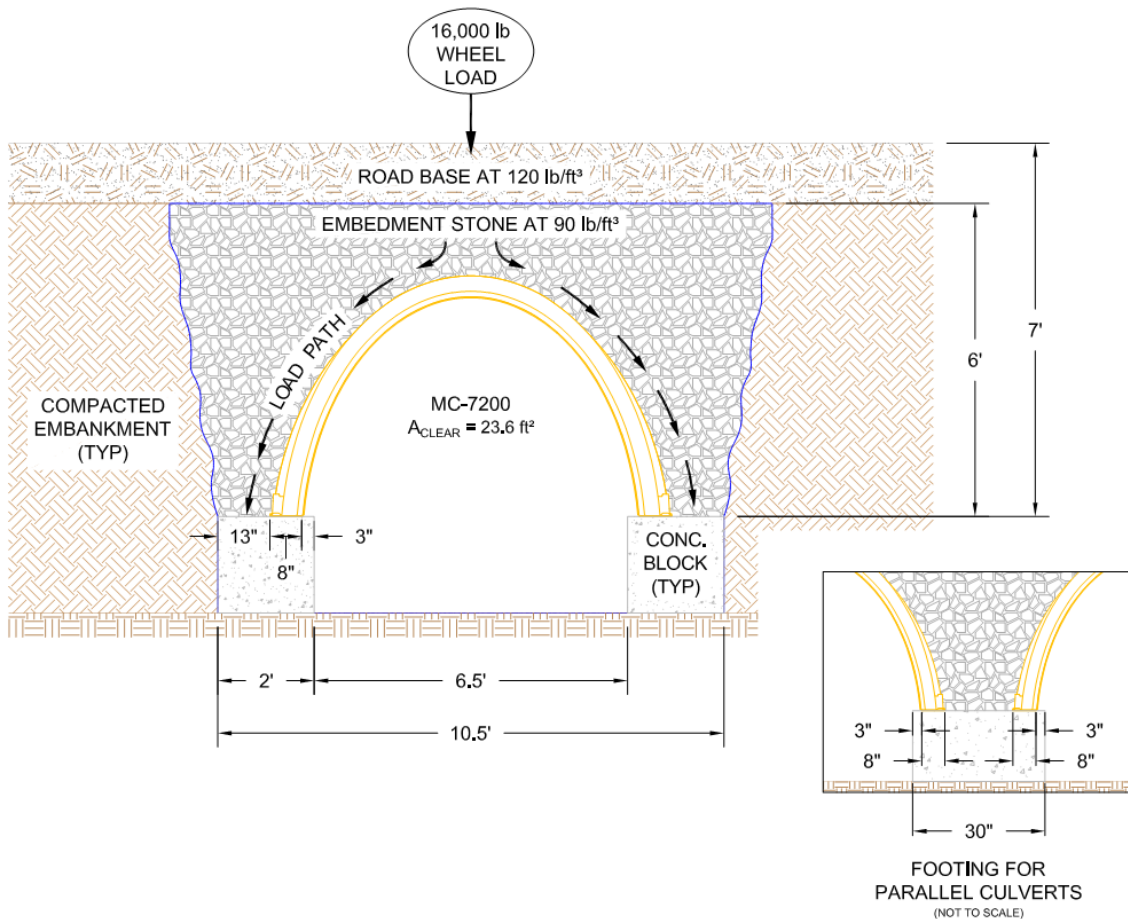
Figure 3 Bottom Crossing Design
