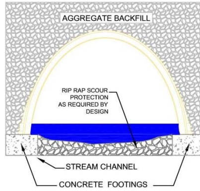
CONCRETE FOOTING OPTION 2: AGGREGATE BOTTOM (FOR LOW FLOW APPLICATIONS)
