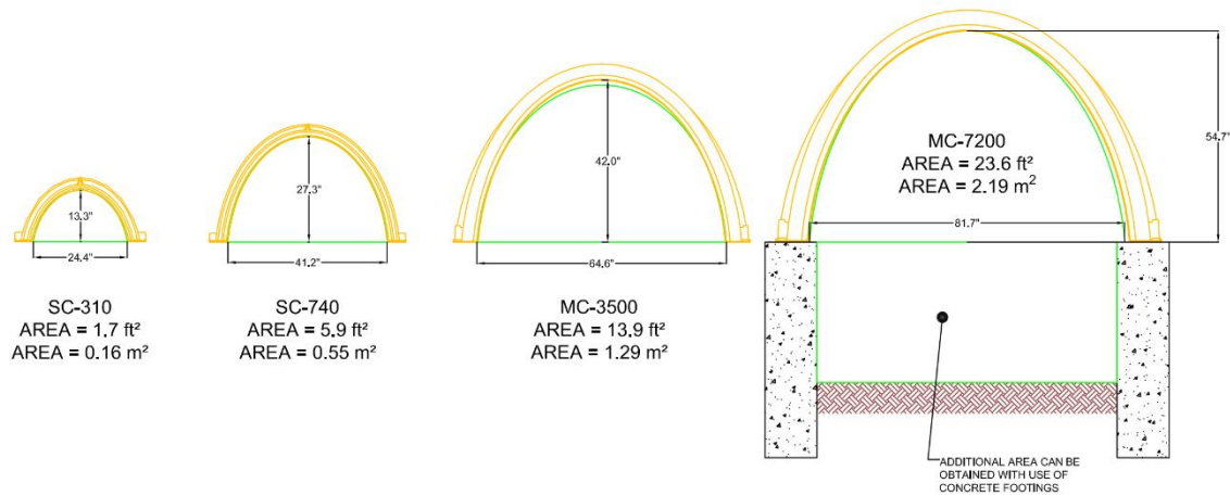
Figure 1 Chamber Dimensions and Open Area
