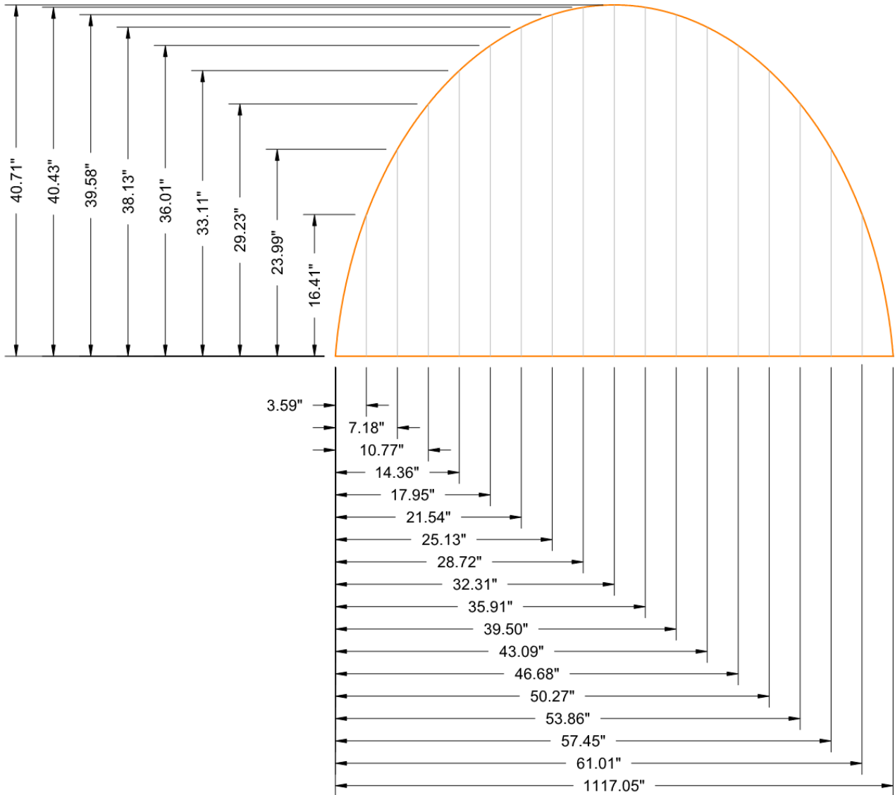
Figure 5 MC-3500 User Defined Shape
