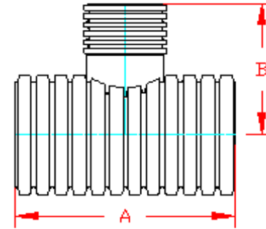
PLAIN END
