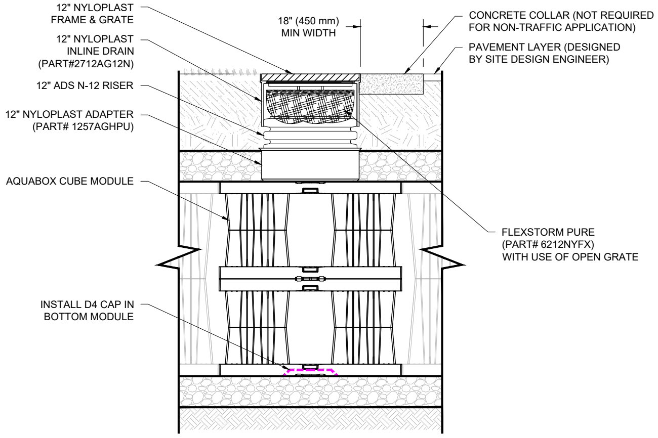
AQUABOX INSPECTION PORT INLET W/FLEXSTORM DETAIL NTS
