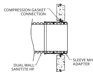
Compression Gasket Connection to Dual Wall Pipe
