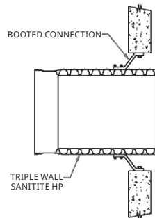
Boot Connection to Triple Wall Pipe
