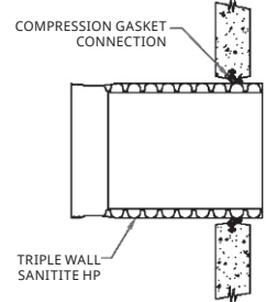
Compression Gasket Connection to Triple Wall Pipe
