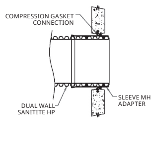
Compression Gasket Connection to Dual Wall Pipe
