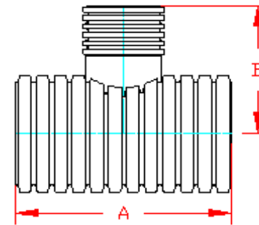
PLAIN END
