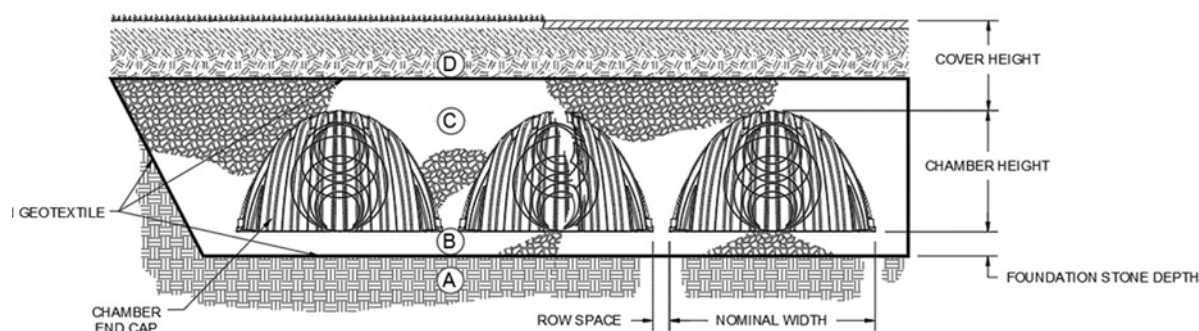
Figure 1: Typical Cross-Section of StormTech System
