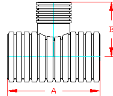
PLAIN END
