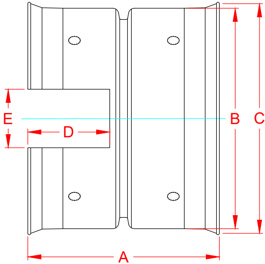
BELL-BELL ADAPTER FOR 6 - 10 IN (150 - 250 mm) PIPE DIAMETER
