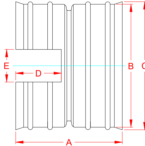
ST CLEATED EXTERNAL ADAPTER FOR 12 - 24 IN (300 - 600 mm) PIPE DIAMETER
