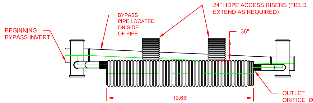
PROFILE VIEW
