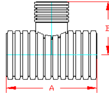
PLAIN END
