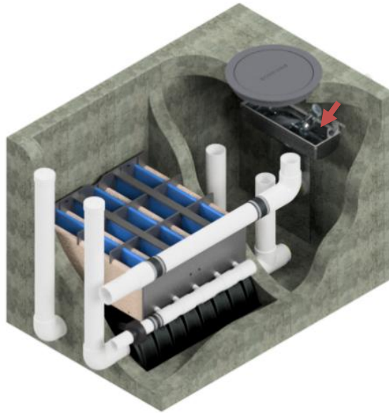
Figure 2: Water begins to inlet into unit and is filtered through the FlexStorm.
