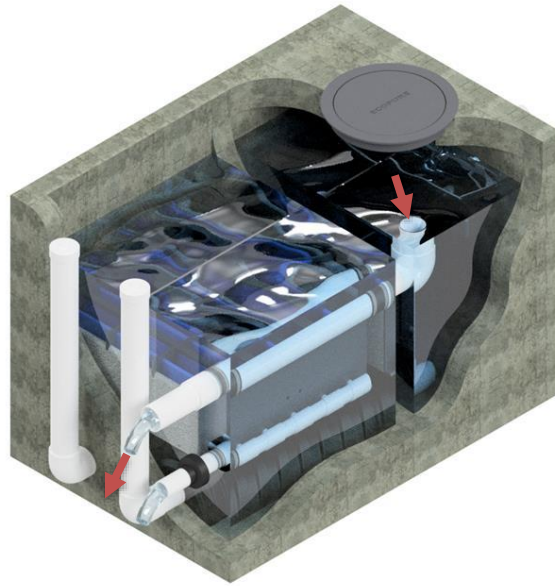
Figure 5: Influent exceeds inlet capacity and exits the system via bypass pipe.
