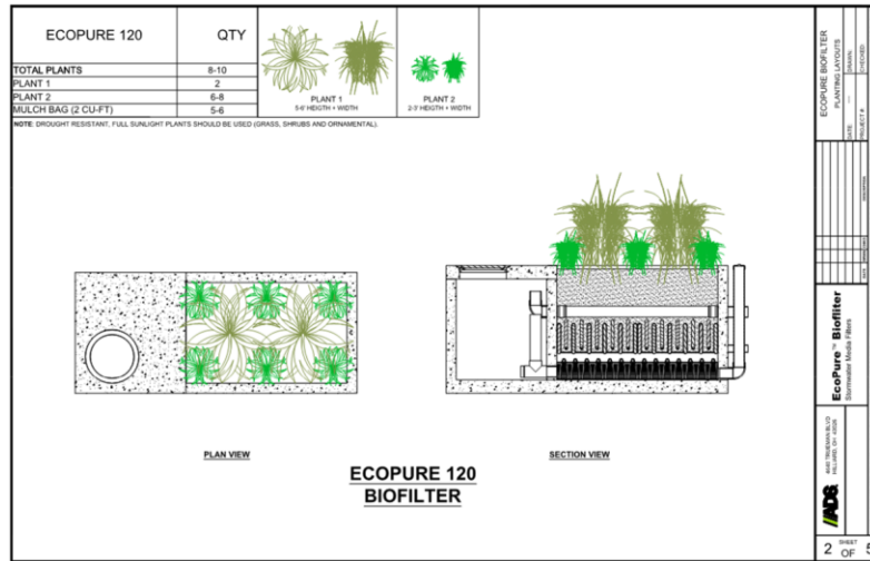
Figure 8: Example plant layout on an EcoPure 120.
