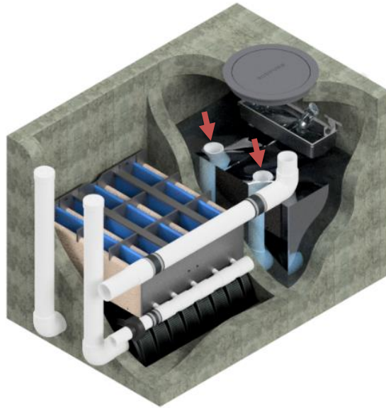
Figure 3: Influent backs up in the unit until it crests the inlet risers.
