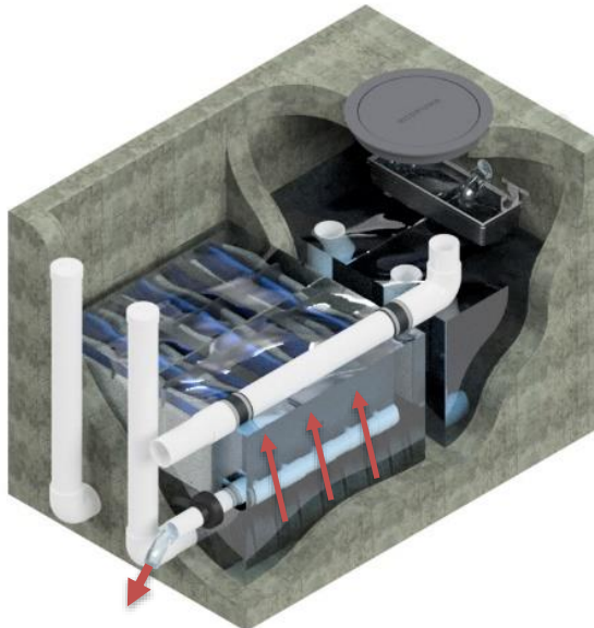
Figure 4: Treated influent ponds in the treatment bay following filtration as it waits to exit through the PVC manifold.
