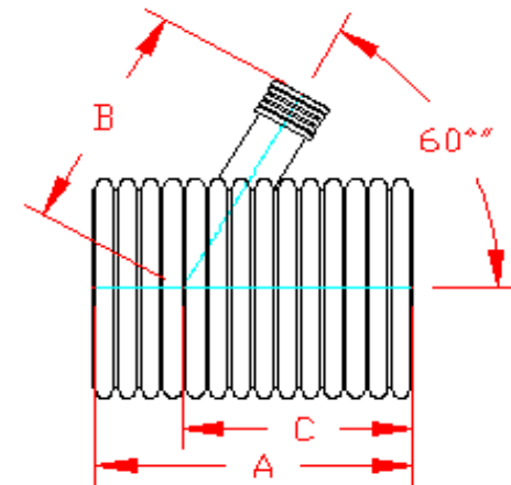
PLAIN END
