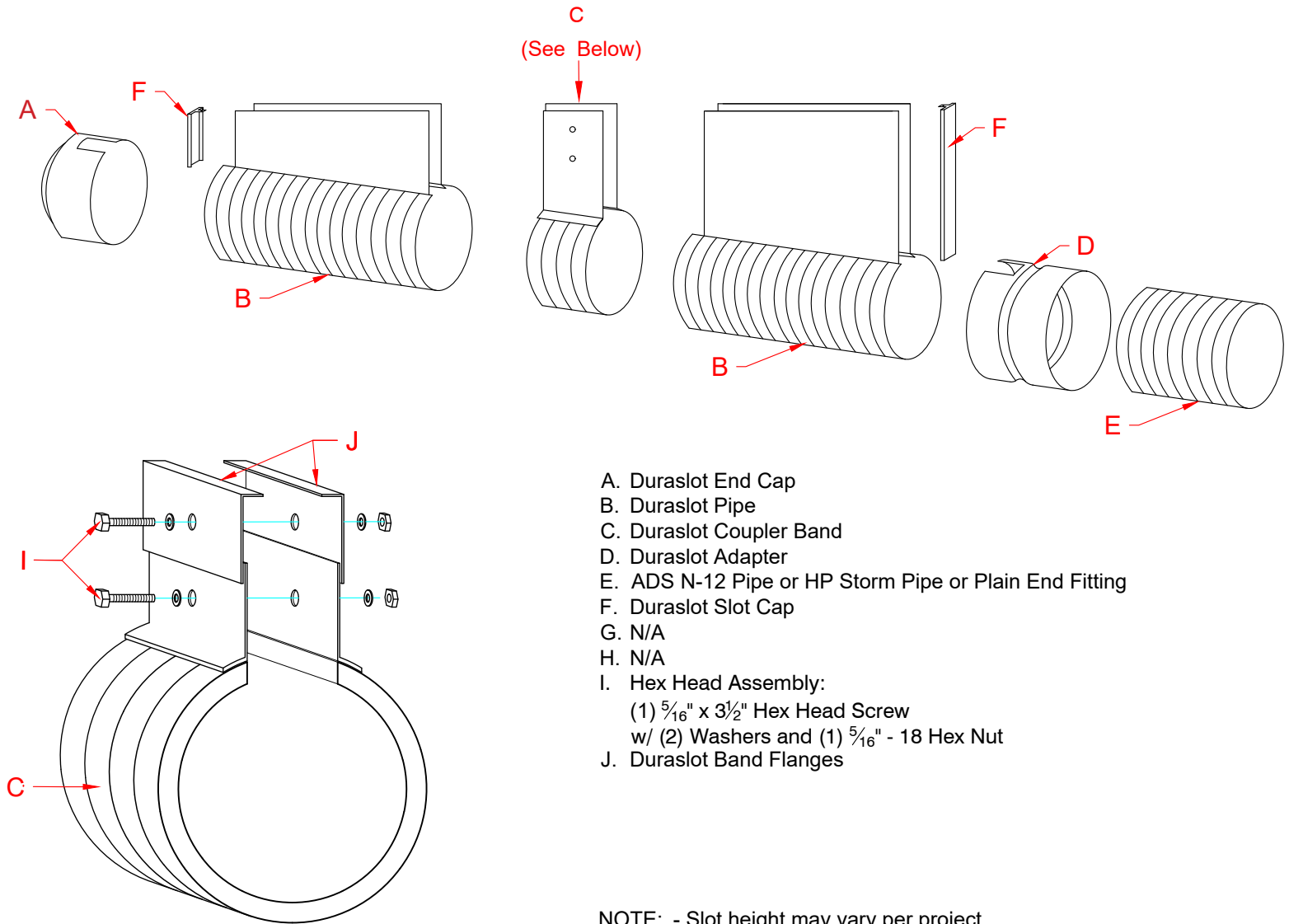
DURASLOT COUPLER BAND (C) HARDWARE ASSEMBLY
