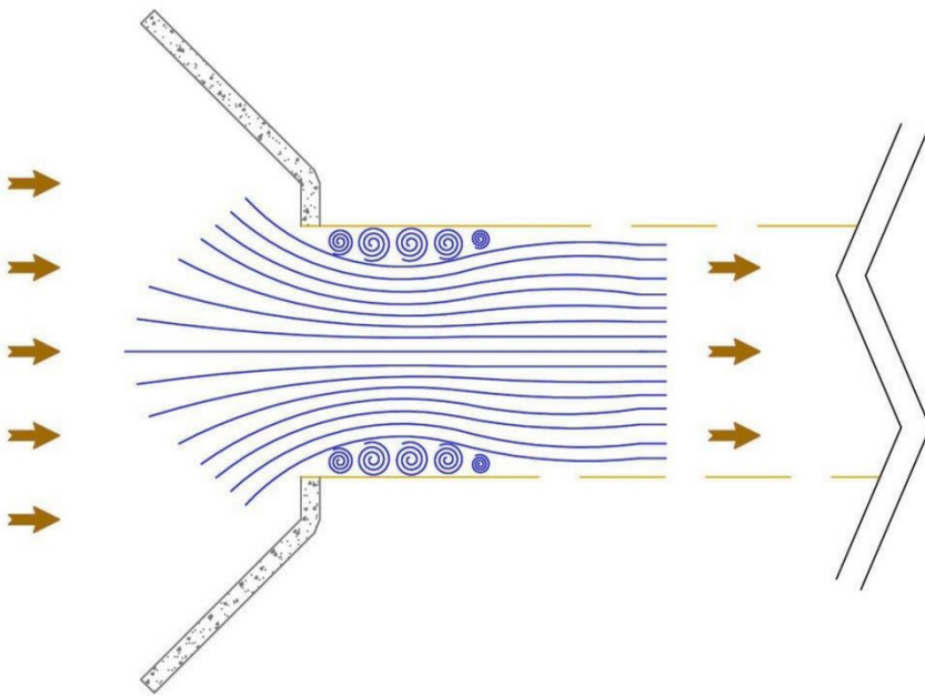
Figure 4: Contraction Scour
