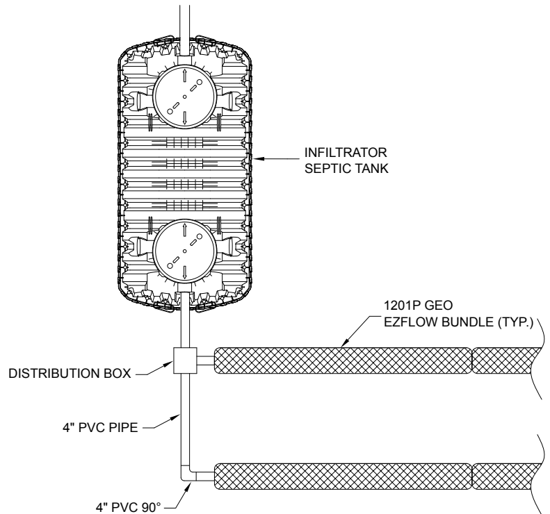
TYPICAL PLAN VIEW (not to scale)
