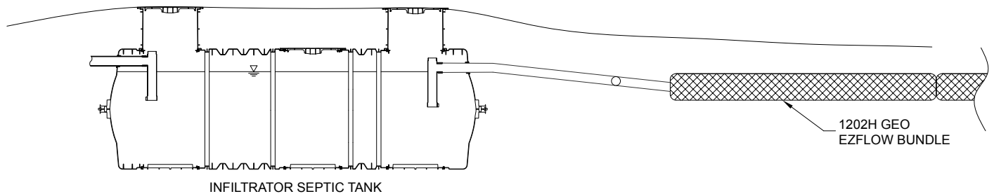
TYPICAL SIDE VIEW (not to scale)
