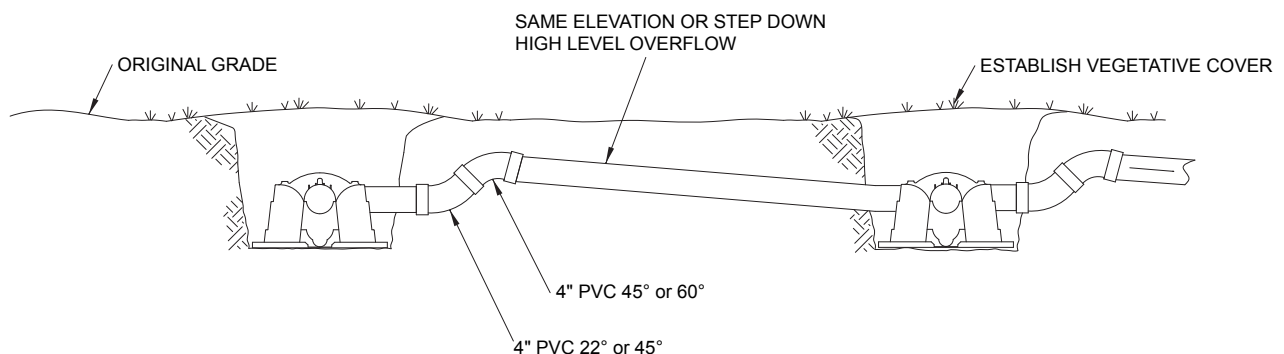
Typical SERIAL DISTRIBUTION SYSTEM ON LEVEL TERRAIN - CROSS SECTION (not to scale)
