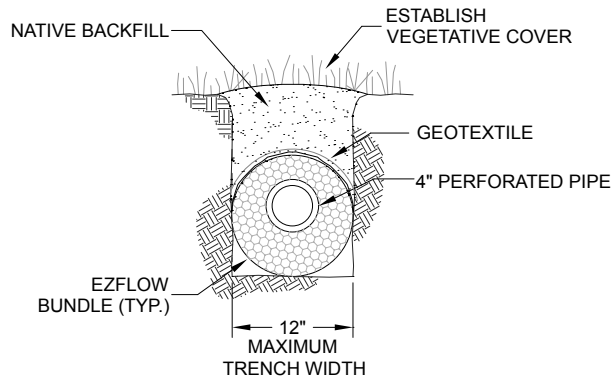
TYPICAL CROSS SECTION (not to scale)
