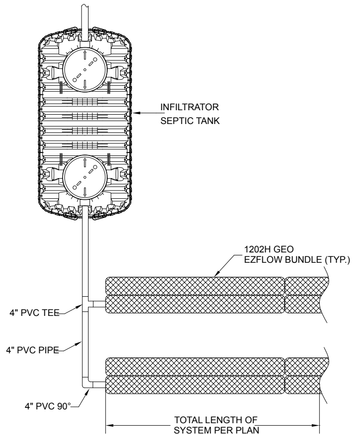
TYPICAL PLAN VIEW (not to scale)
