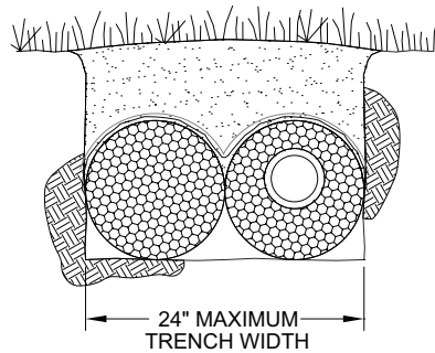
TYPICAL CROSS SECTION (not to scale)
