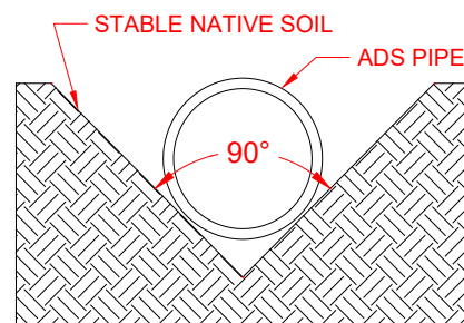
Figure 1 V-Bottom Trench
