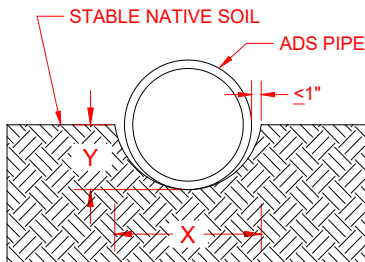
Figure 2 Rounded Trench Installation
