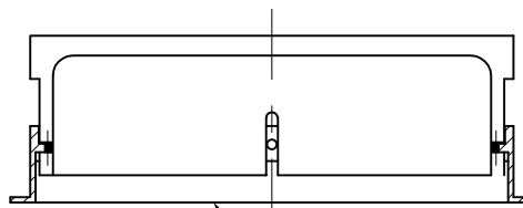
2' X 3' CURB INLET LOCKING FRAME & HOOD 3099CGRFHL
