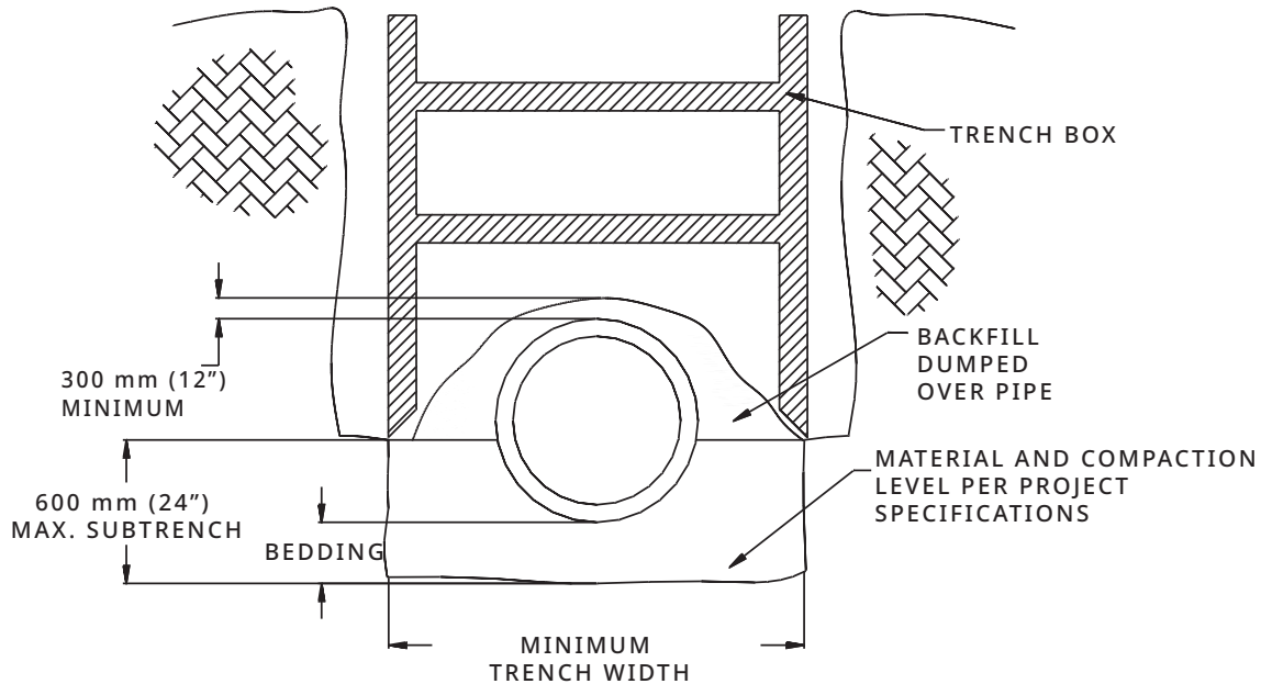
Figure 2: Subtrench Installation
