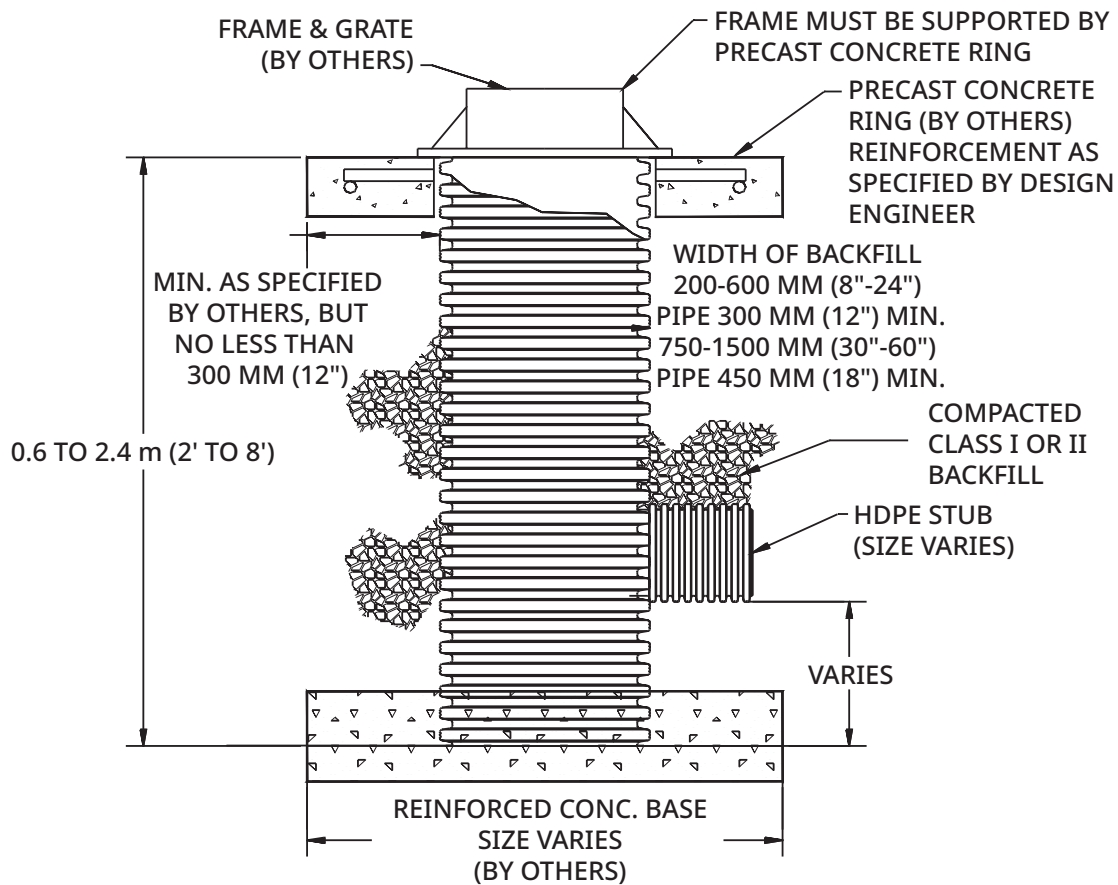
Figure 6: Vertical Riser
