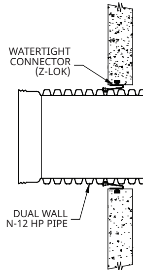
TYPE 4 WATERTIGHT USING MECHANICAL CONNECTOR
