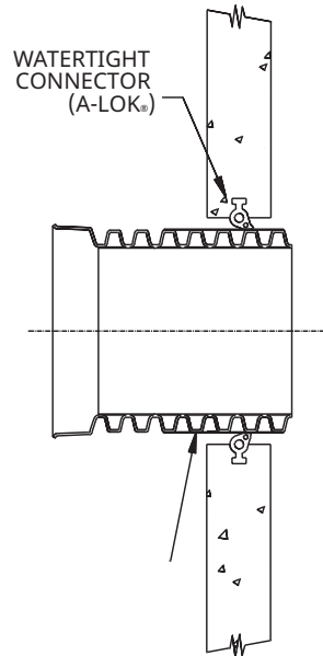
TYPE 2 WATERTIGHT USING PRE-FABRICATED ADAPTER
