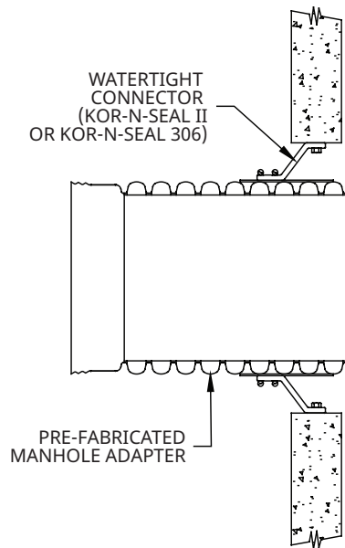
TYPE 1 WATERTIGHT USING PRE-FABRICATED ADAPTER
