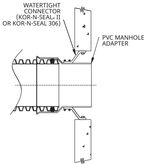
TYPE 3 WATERTIGHT USING PVC MANHOLE ADAPTER
